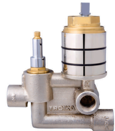
AL 343A Concealed Body For Single Lever Diverter, 35mm Cartridge With Lever Assembly But Without Exposed Parts
